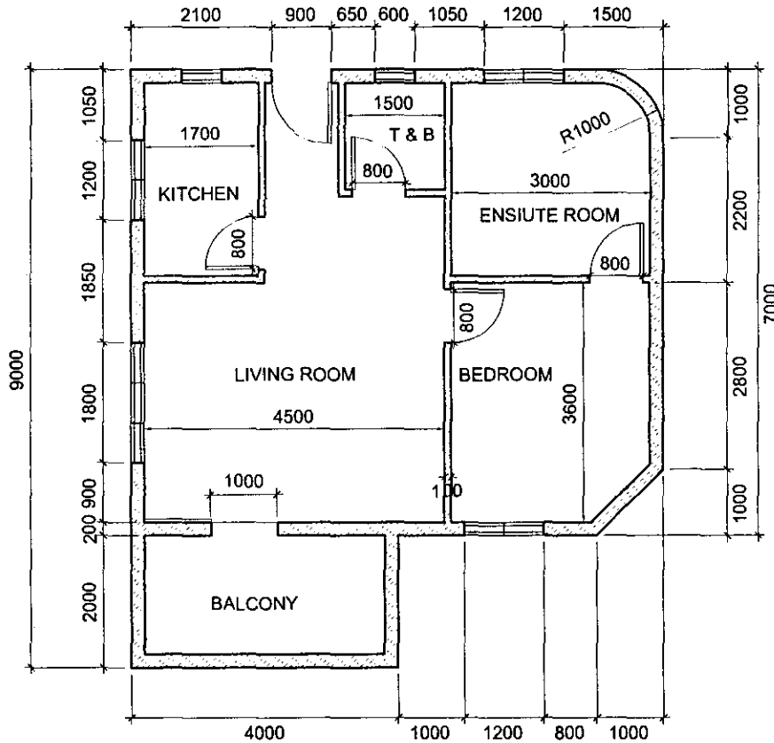
FLOOR PLAN
