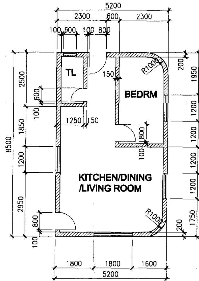
SIMPLE FLOOR PLAN
