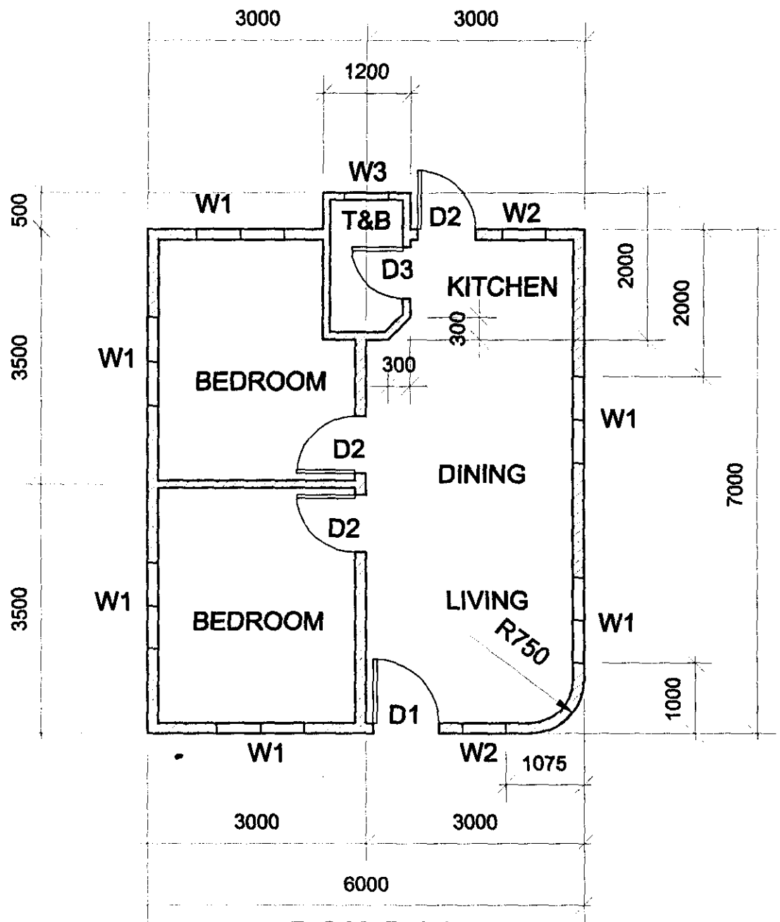
FLOOR PLAN
