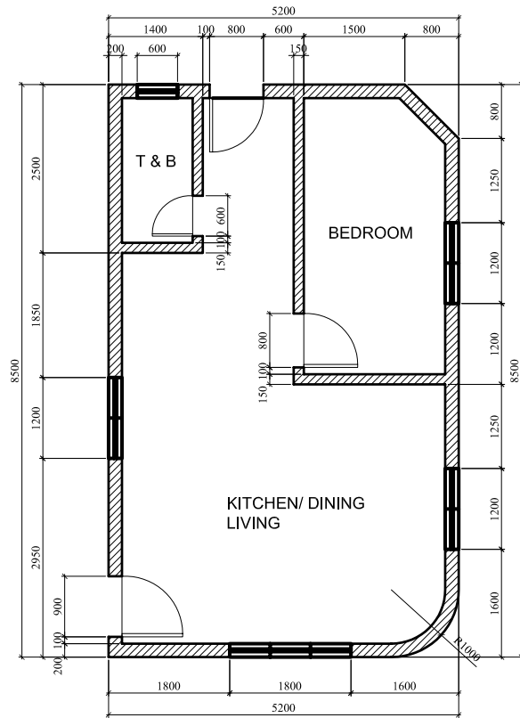
FLOOR PLAN
